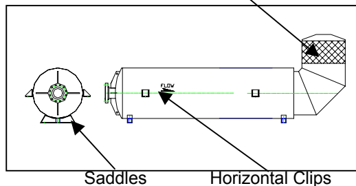
Elbow outlet with Weatherhood
